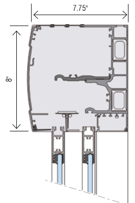
Telescopic Casing
