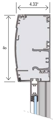
Standard Casing
