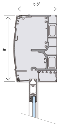
Reinforced Casing
